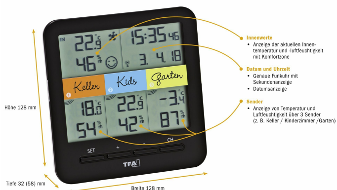
KLIMA@HOME Funk-Thermo-Hygrometer
